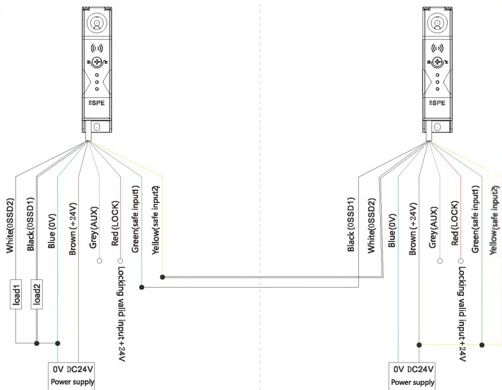
SLR11 advanced type(NPN, no cascade)
