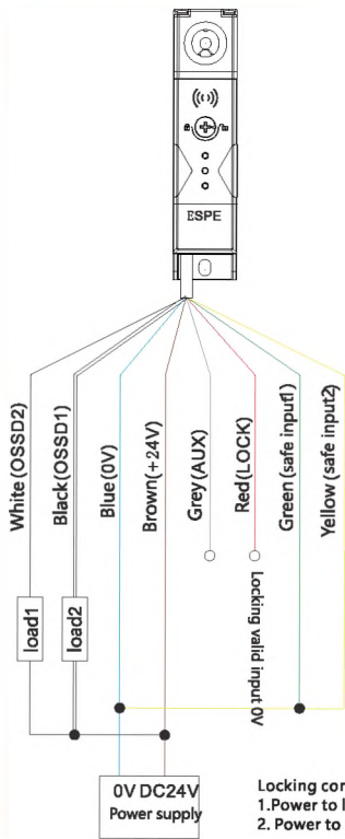
SLR11 normal type(NPN, cascade)
